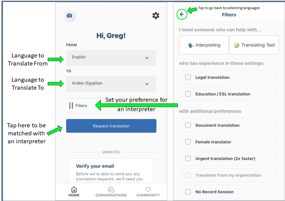
Translating in Tarjimly
